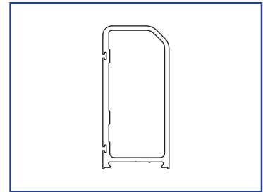
US01-0406-LLCL Medium Stile Besam Rail
