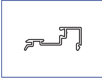
US01-0418-LLCL 1/4" Gutter
