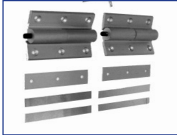
50-15-022CL Hinge Kit, HD, Surface Mount (MAC 10), CL, Bi-Way
