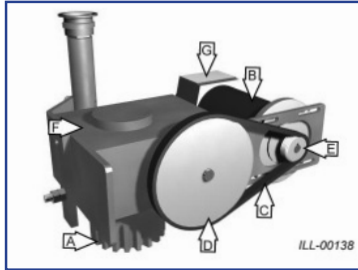
331001167 Drive Unit Complete, RD3/RD4
