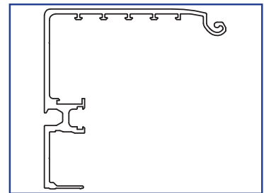
US01-0295-LLMF Beam **
