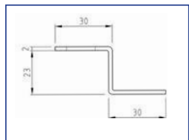
245834 Z Bracket, Ceiling
