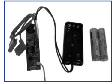
USCMTX9 Transmitter, Wall Switch, 915 MHz
