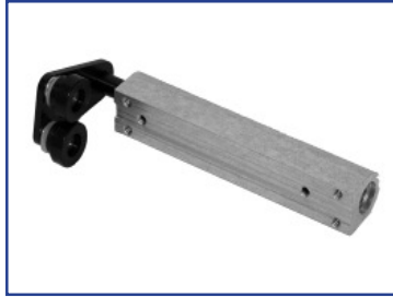
US15-0644-03 Roller Guide Assembly, FSL, Long Axle
