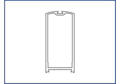
US01-0409-LLCL Medium Stile Single Fuzz, Nose Rail
