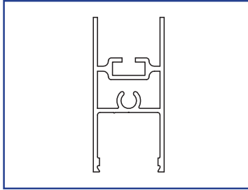
US01-0455-LLCL 2 3/16" Top Rail
