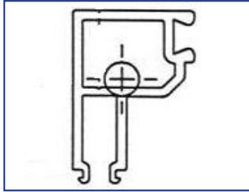
US01-1604-LLCL Non-impact Snap, CL
