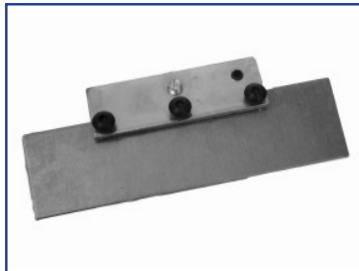
D4204108593 Catch, Panic, Clapper Plate & Magnet
